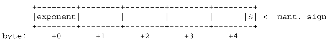
Figure 2. Internal Representation of REAL Numbers
